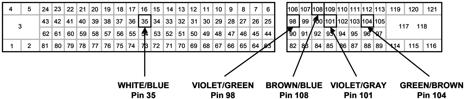
ECU Connector Diagram – Wire Side View
